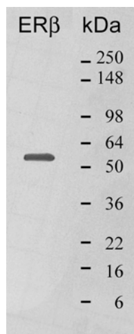
Figure 1: Western blot of ER \beta using ECL detection. Final concentration of antibody was 1.0 \mu g/mL.
